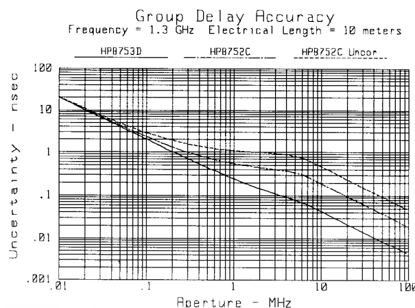
Group Delay Accuracy vs. Aperture
